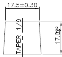
POSITIVE TERMINAL
