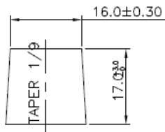
NEGATIVE TERMINAL
